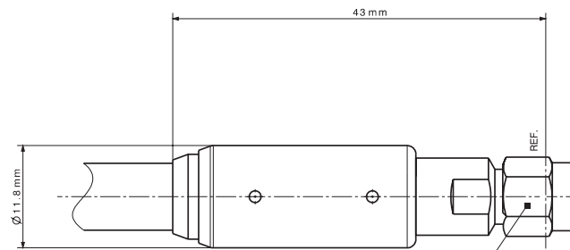
2.92 mm male (SF_11_SK-504)
