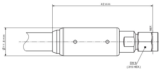
2.4 mm male (SF_11_PC24-504)
